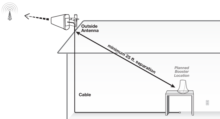
Omni Yagi Antenna Install Illustration
